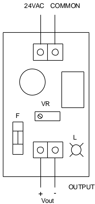
WIRING DIAGRAM
