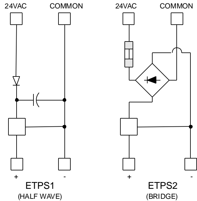
SIMPLIFIED SCHEMATICS
