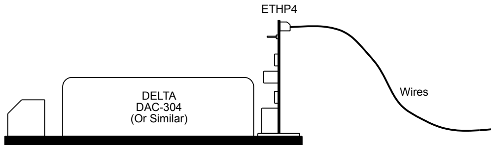
Recommended Mounting
